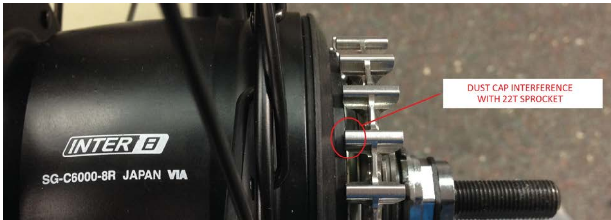
Figure 1: Interference between A-spec dust cover and 22t CDX Sprocket
