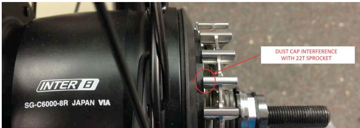
Figure 1: Interference between A-spec dust cover and 22t CDX Sprocket
