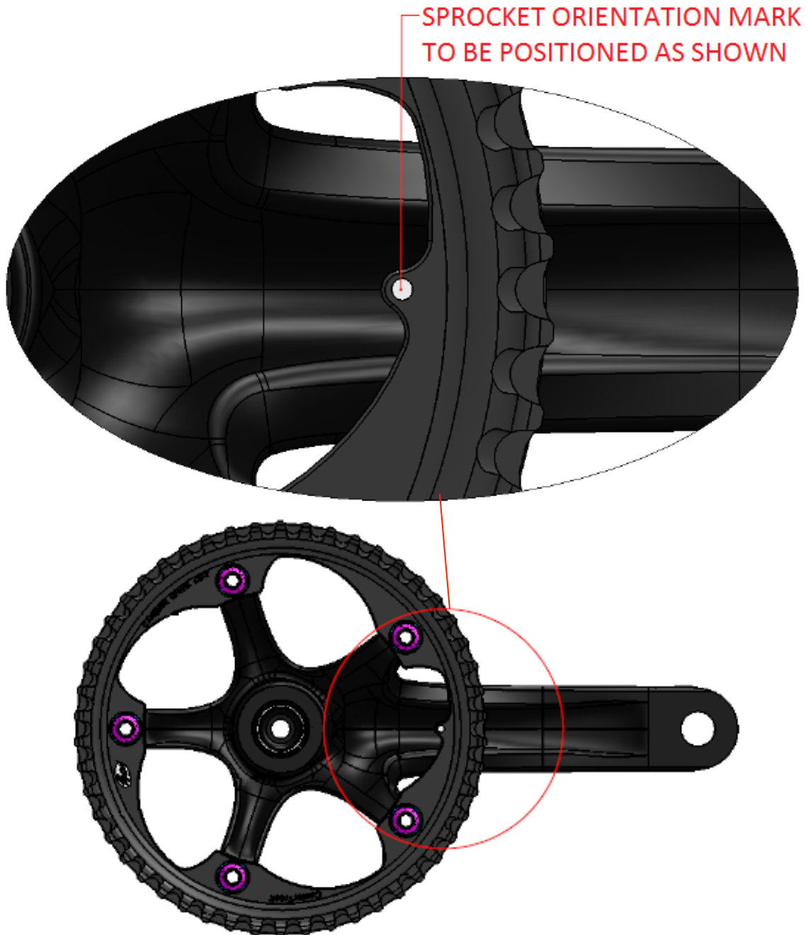
Figure 1: Tab mounting location for correct sprocket orientation.
